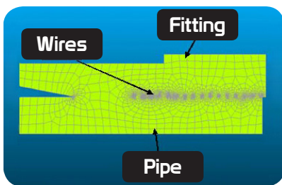
2D THERMAL ANALYSYS (THROUGH ANSYS)
