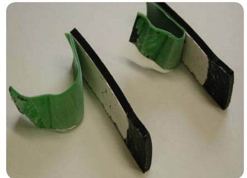
PEEL TEST ON OILTECH SAMPLES
